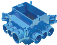
Mud box with one-gang ring
