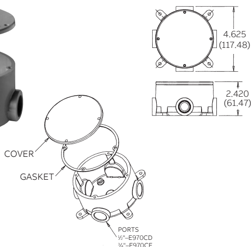
Conduit bodies Type X with cover
